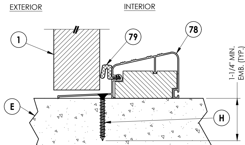
3 VERTICAL CROSS SECTION 5 Outswing configuration
