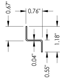
12 MULLION Z BRACKET
