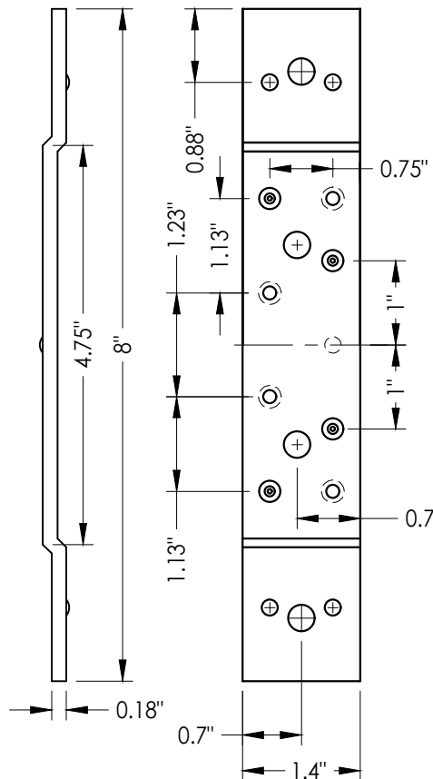
23 STANDARD (SHORT) DOOR HINGE Reinforcement middle and bottom hinge
