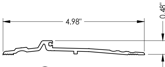
40 THRESHOLD
